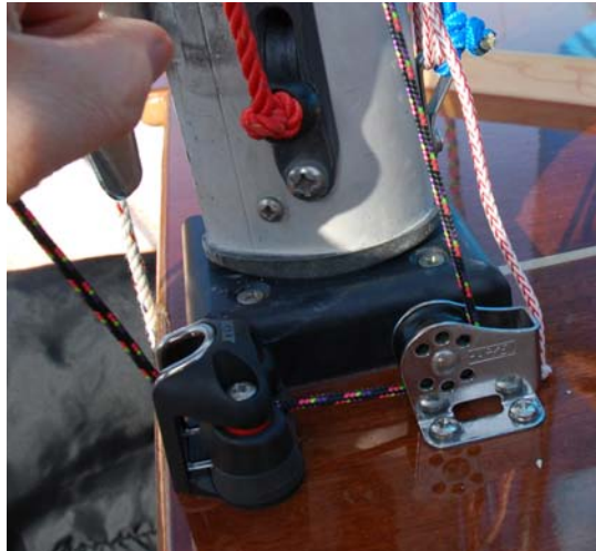
Rope from pole goes through upright block and then to cleat for adjustment by crew
